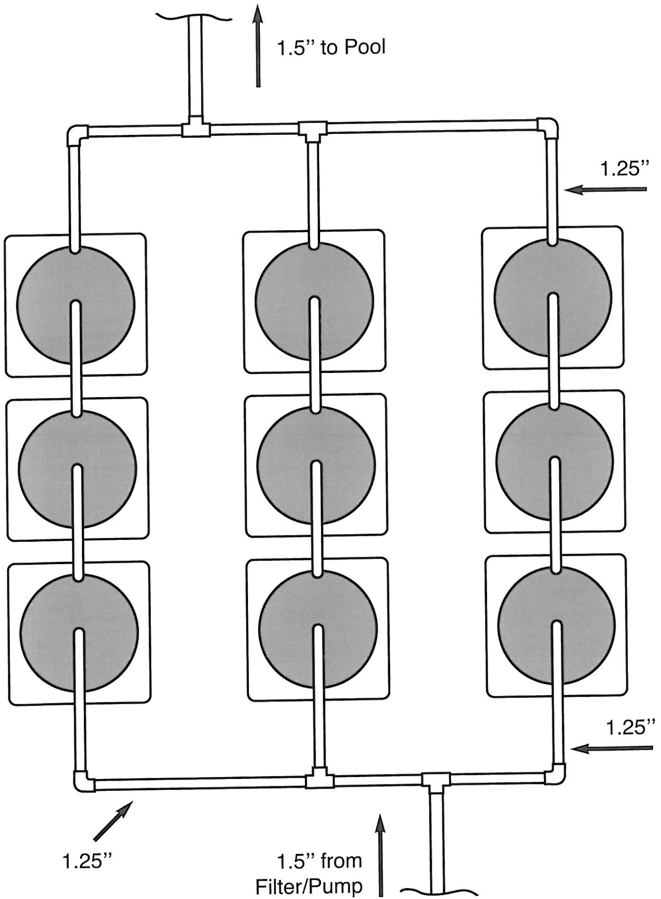
Diagrammatic Layout of Solar Pods (view of underside)
